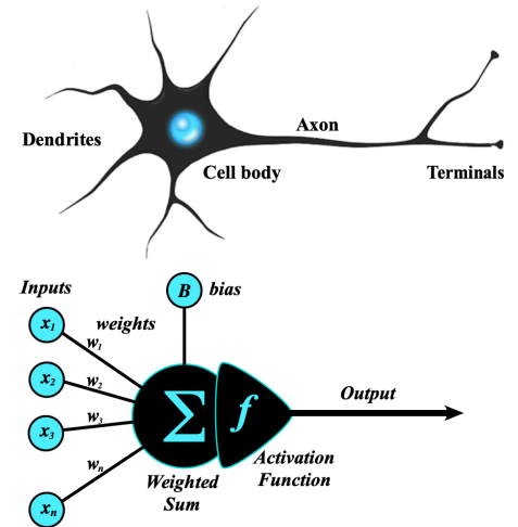
Figure 2.4: Neuron structure [31]
